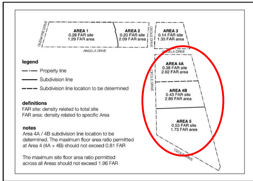
FIGURE 5 – MAXIMUM FARs PERMITTED BY DENSITY TRANSFER - ORIGINAL
