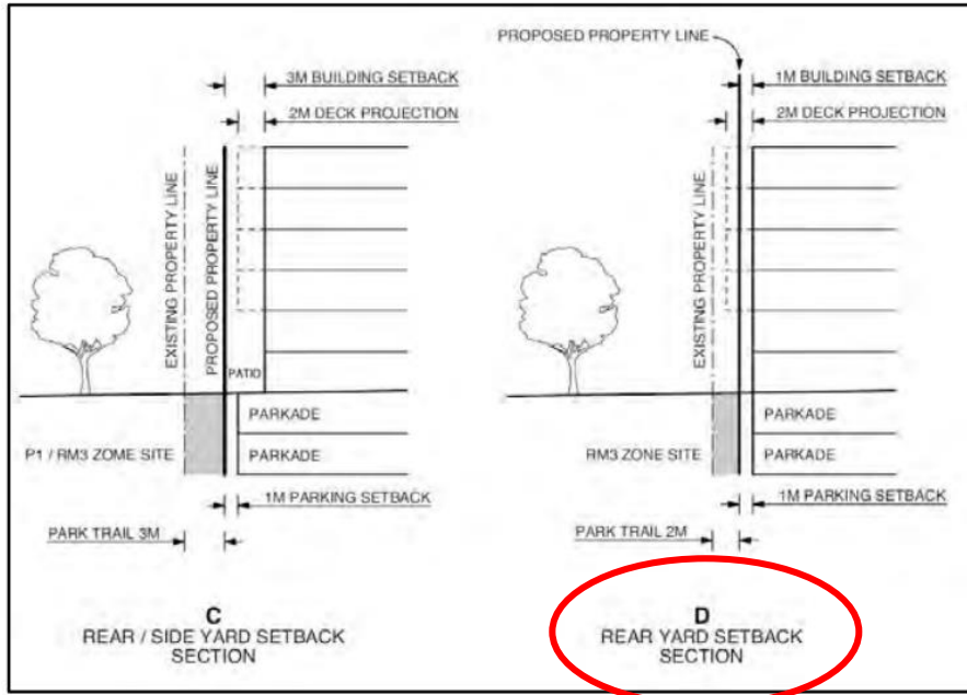
FIGURE 9 – BUILDING SETBACK DETAILS (as to Section D only) - ORIGINAL
