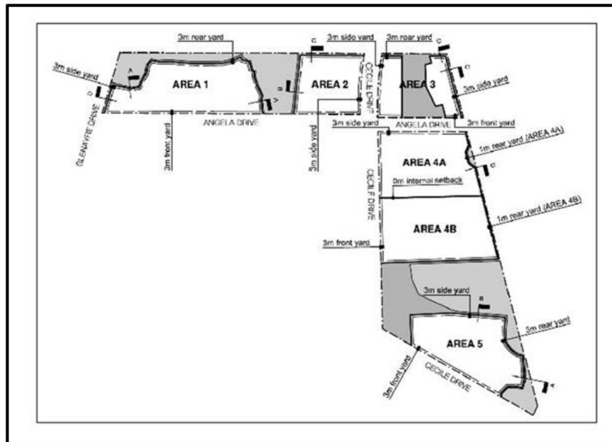
FIGURE 7 – BUILDING SETBACKS - ORIGINAL
