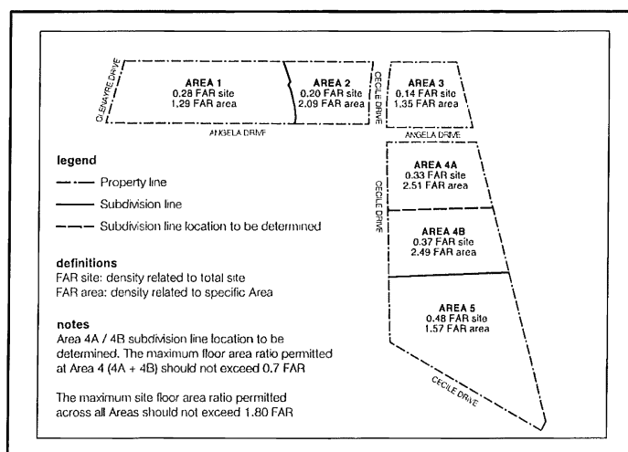
Figure 3 – Maximum Permitted Floor Area Ratios
