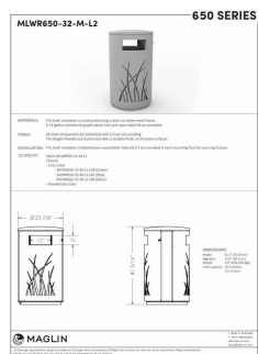
TRASH BIN SURFACE MOUNT BY MAGLIN; MLWR650-32-M-L2
