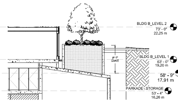
04 SECTION 4 L19 SCALE: 3/16"=1'-0"
