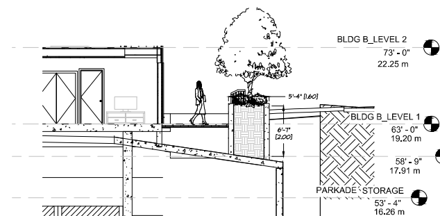
03 SECTION 3 L19 SCALE: 3/16"=1'-0"
