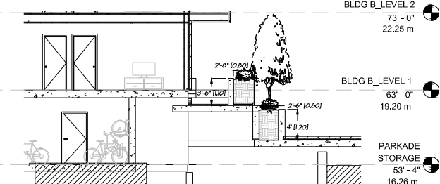
01 SECTION 1 L19 SCALE: 3/16"=1'-0"
