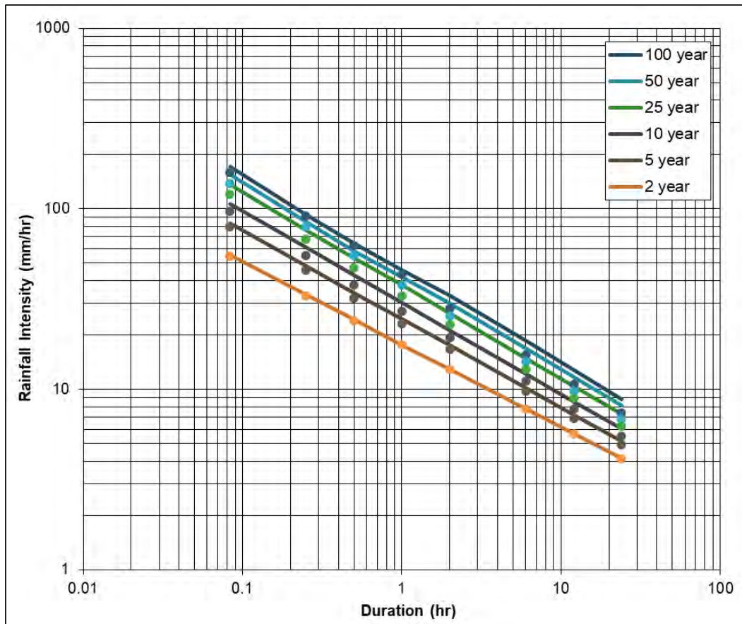
Figure 3: Estimated IDF Curve for PT11 Rain Gauge Climate Change Condition (Year 2050-2100)
