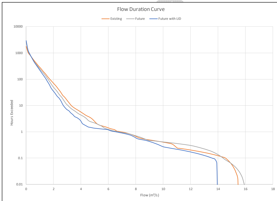
Figure 7: Flow Duration Curve Comparison
