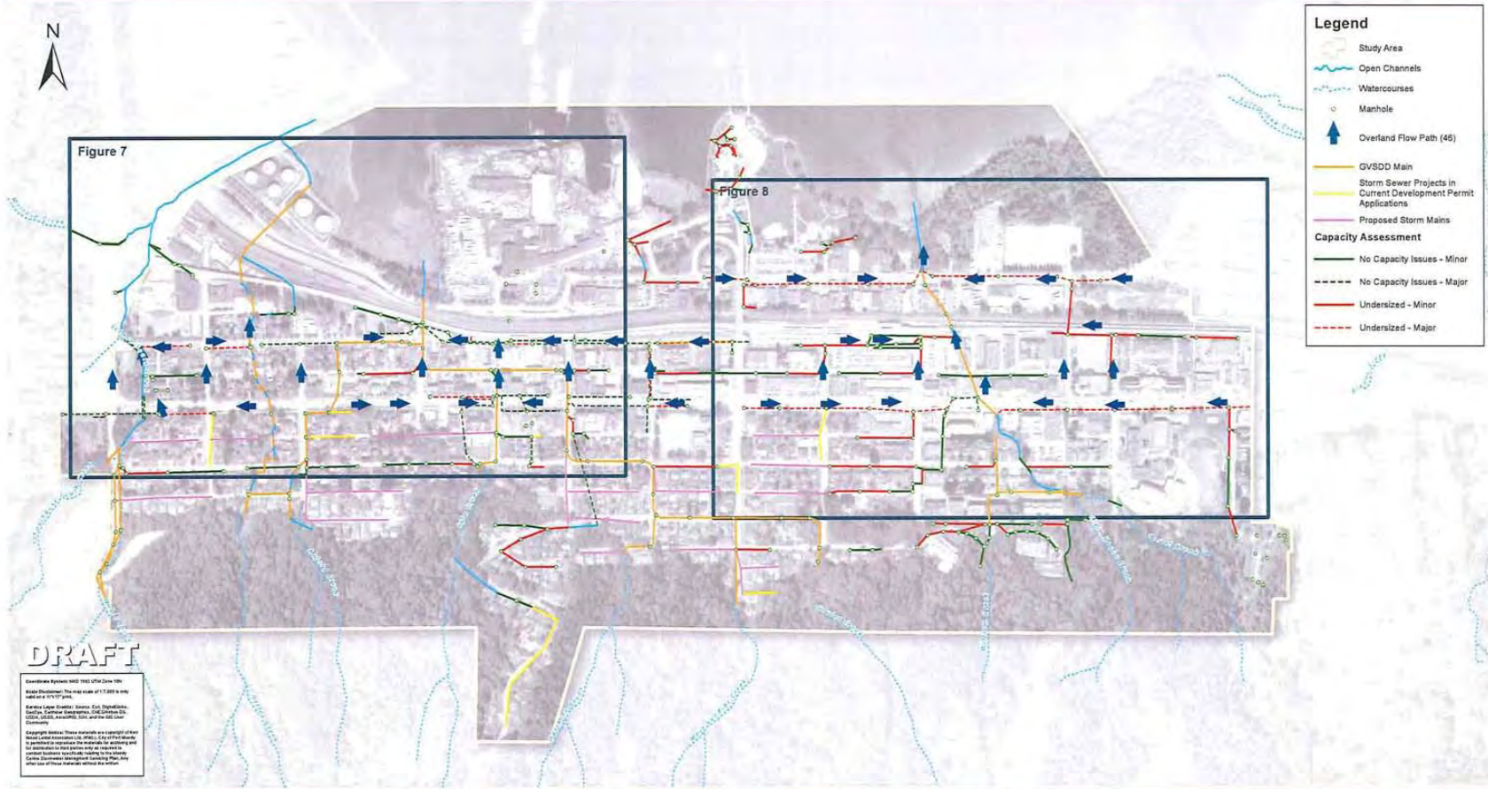
Future Conditions Capacity Assessment (100-year Design Storm with Climate Change) and Overland Flow Path
