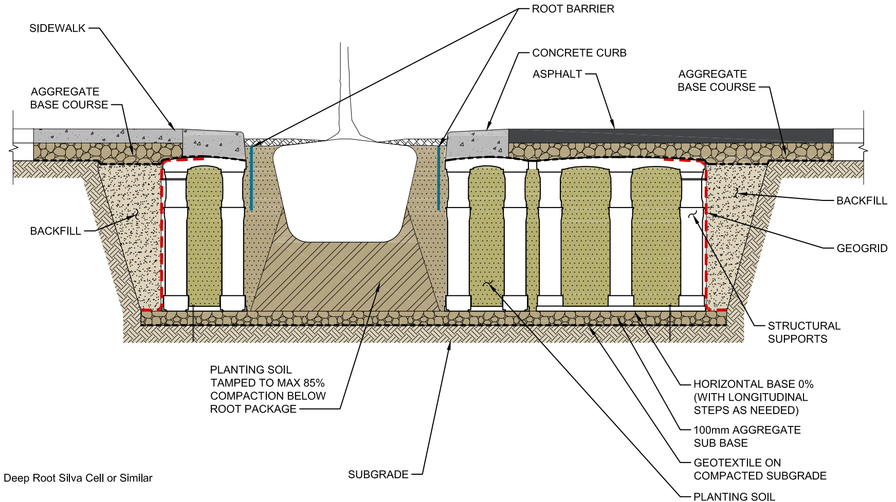
Structural Soil Cell - Section View
